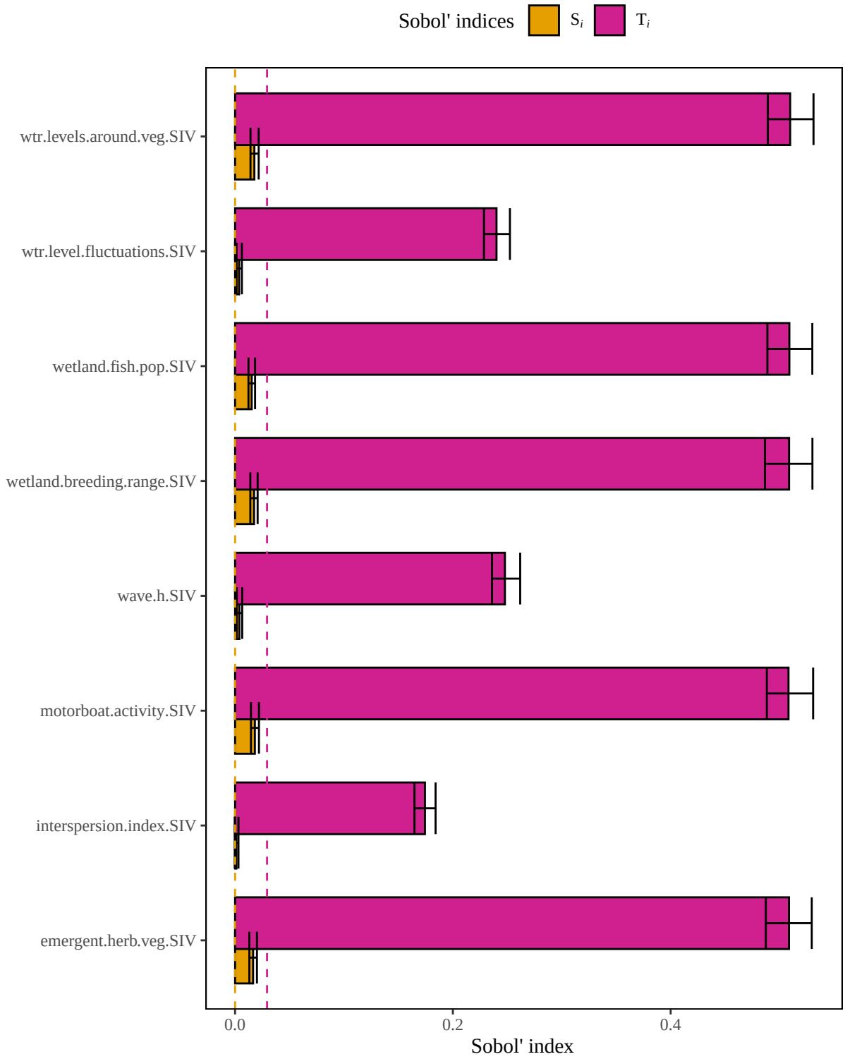
Figure 6. Results of a sensitivity analysis for the westerngrebe model based on a limiting factor structure. Dashed lines represent baseline numerical approximation error for S_i and T_i ( i.e. , dummy variables).
