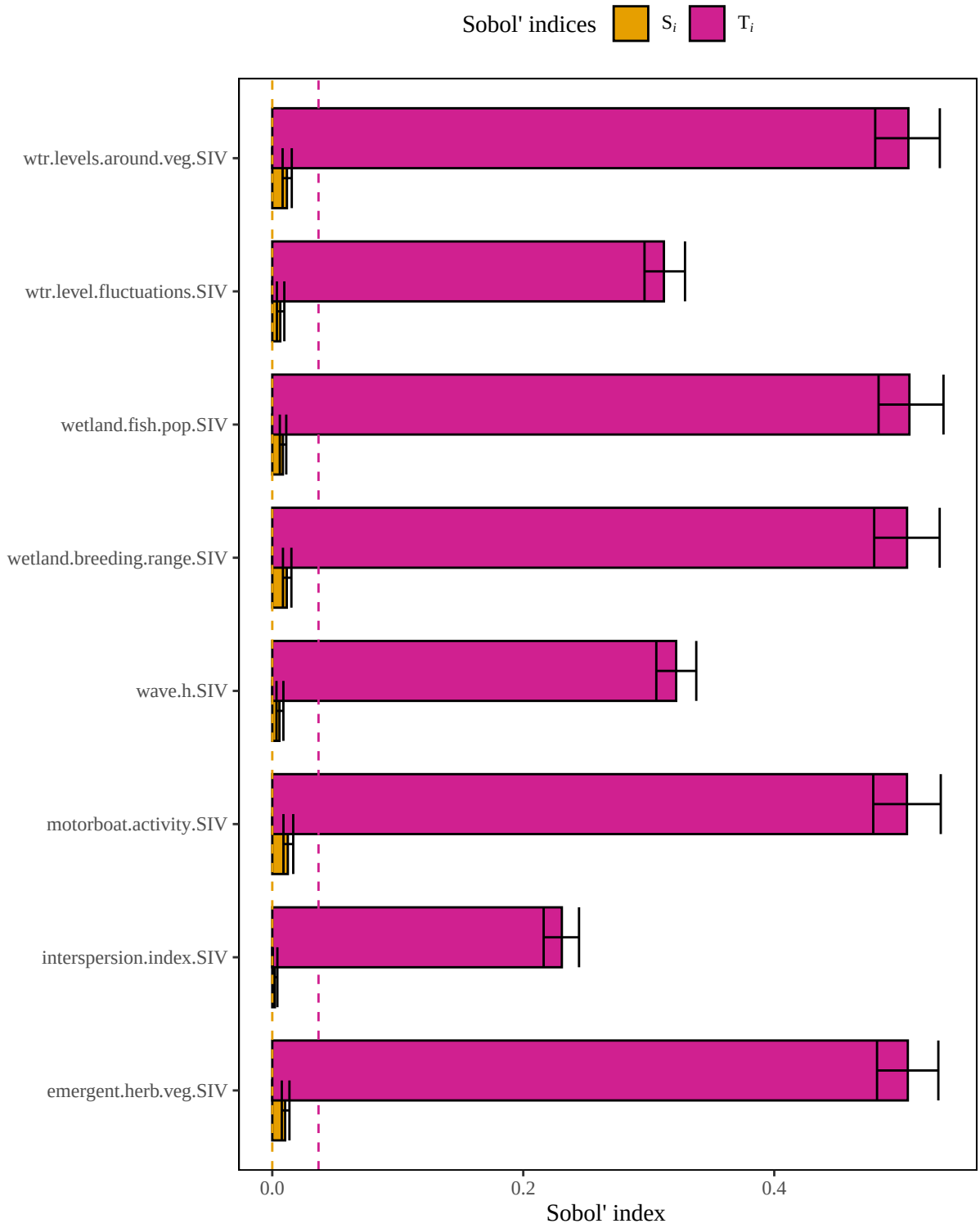
Figure 7. Results of a sensitivity analysis for the westerngrebe model based on a multiplicative mean structure. Dashed lines represent baseline numerical approximation error for S_i and T_i ( i.e. , dummy variables).
